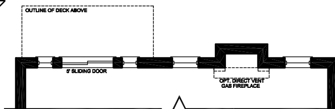
PARTIAL OPT. FIN. BASEMENT FLOOR ELEV. 'A' & 'B' FOR WALK-OUT BASEMENT CONDITION
