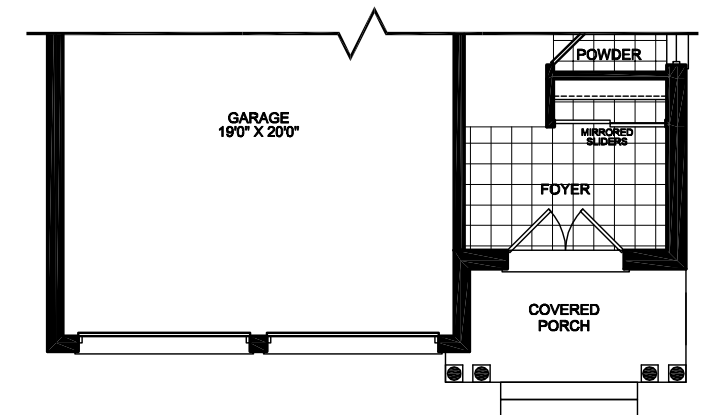
PARTIAL GROUND FLOOR ELEV. 'B'
