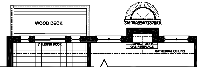
PARTIAL GROUND FLOOR ELEV. 'A' & 'B' FOR WALK-OUT BASEMENT CONDITION
