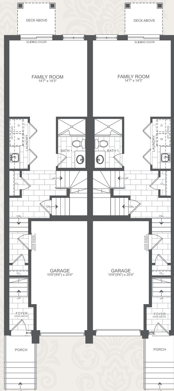
GROUND LEVEL ELEVATION A
